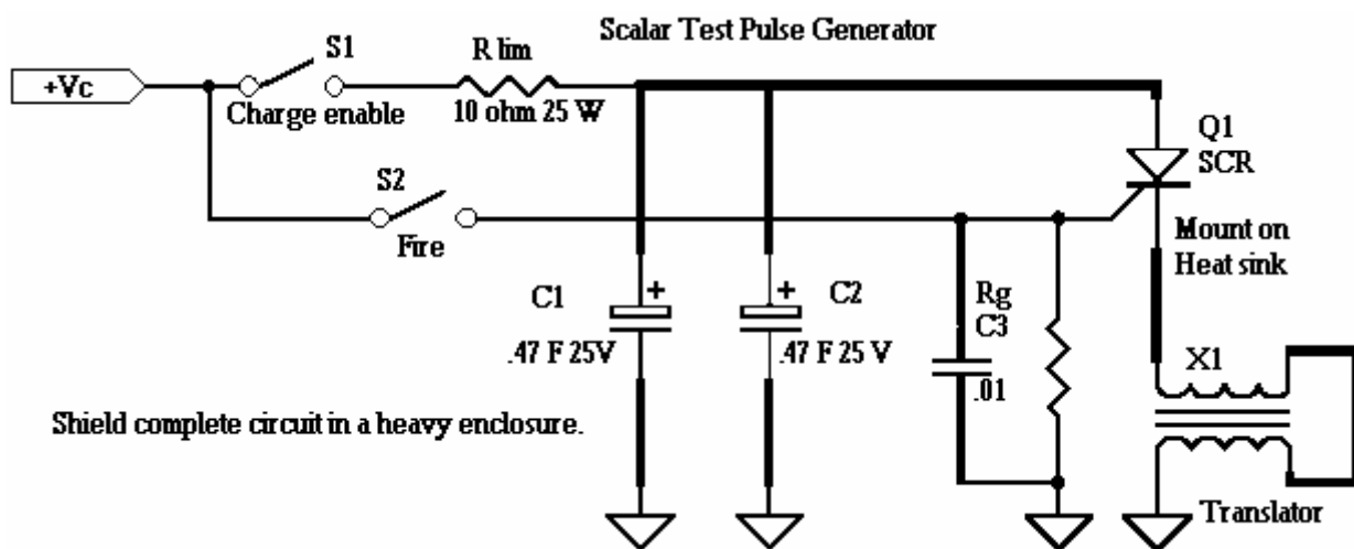
SCHMAT1A.GIF Schematic of Scalar Pulse Generator
